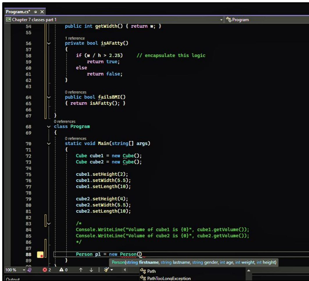
Figure 7.6: Parameterized Constructor Method
